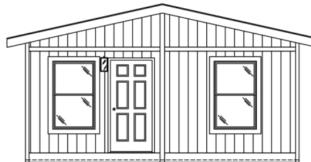
FRONT ENDWALL
