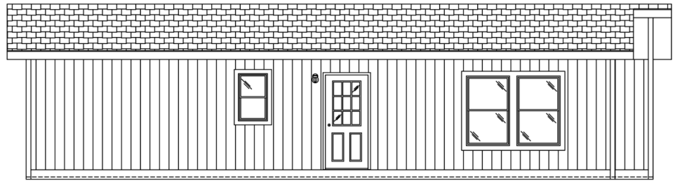
FRONT SIDEWALL
